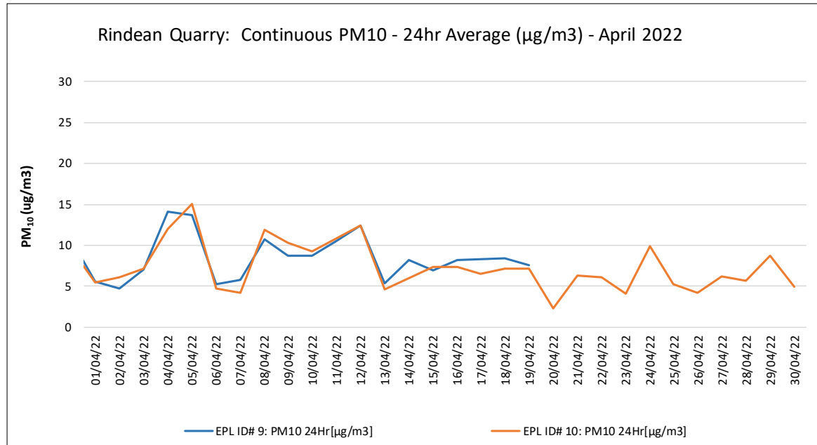
Figure 1: Continuous 24hr Averages – April 2022
