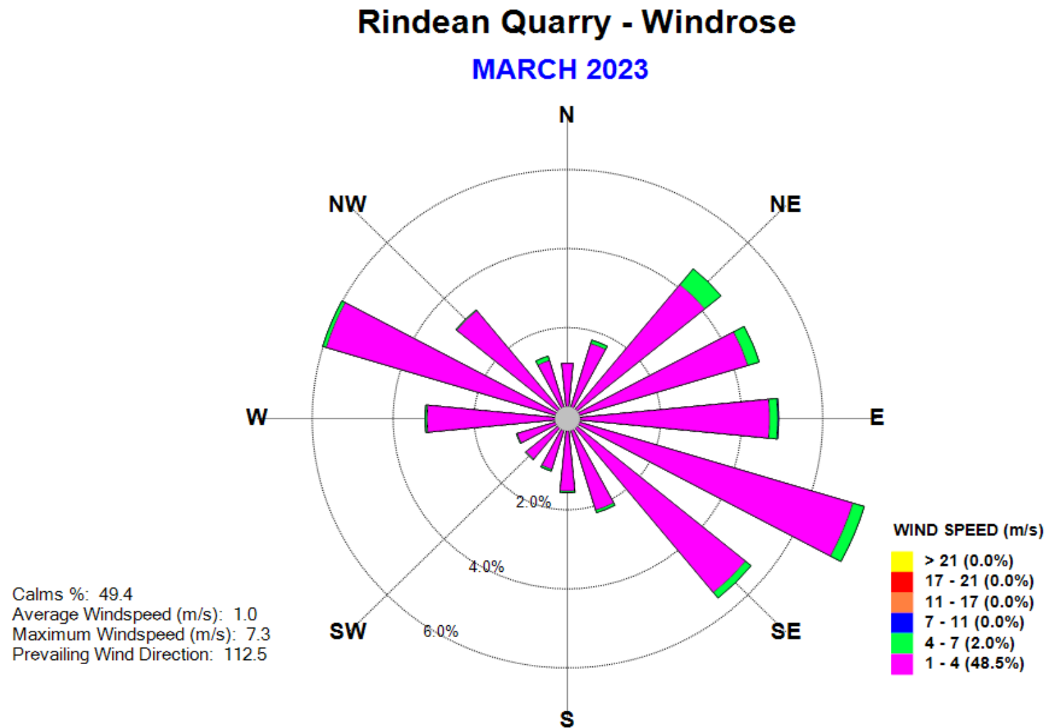
Figure 2: Windrose – March 2023
