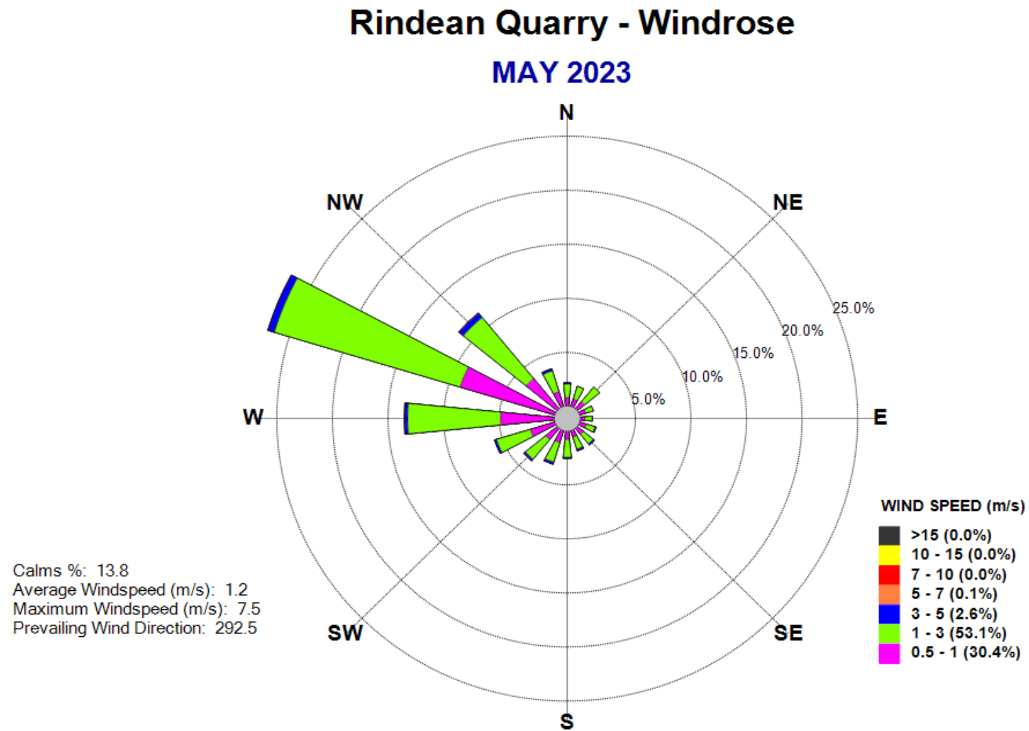
Figure 2: Windrose – May 2023
