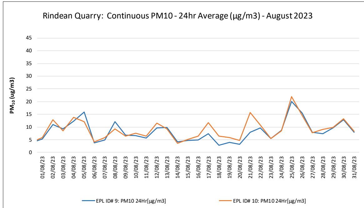
Figure 1: Continuous 24hr Averages – August 2023
