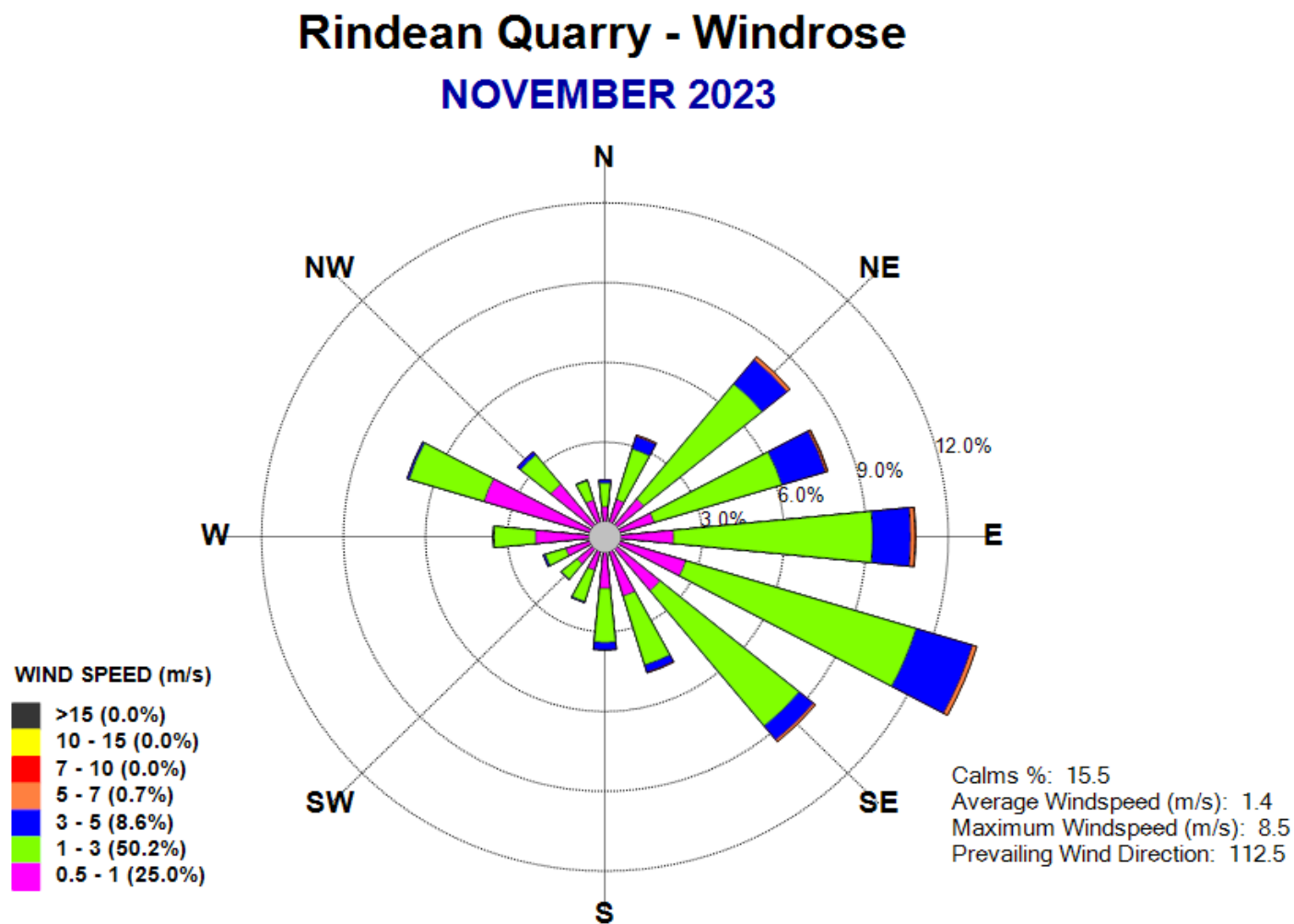
Figure 2: Windrose – November 2023
