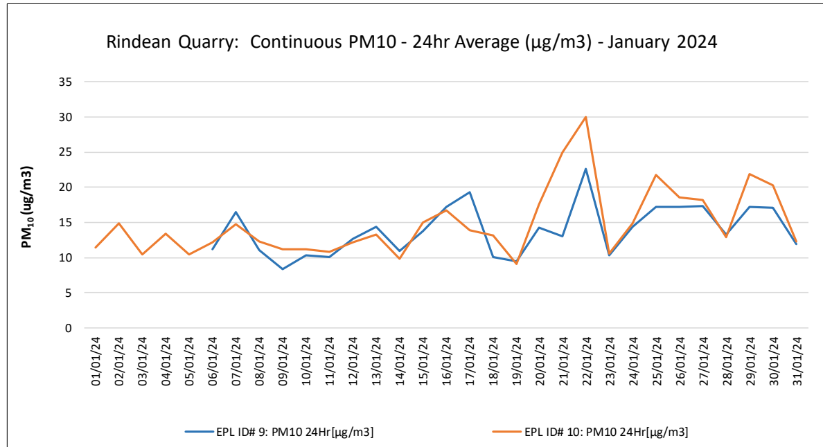
Figure 1: Continuous 24hr Averages – January 2024
