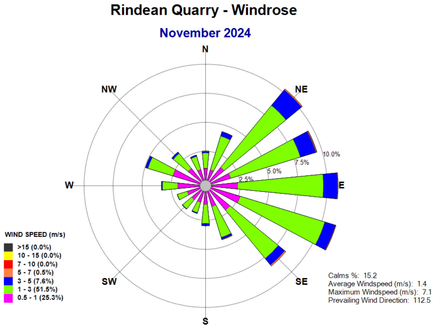
Figure 2: Windrose – November 2024
