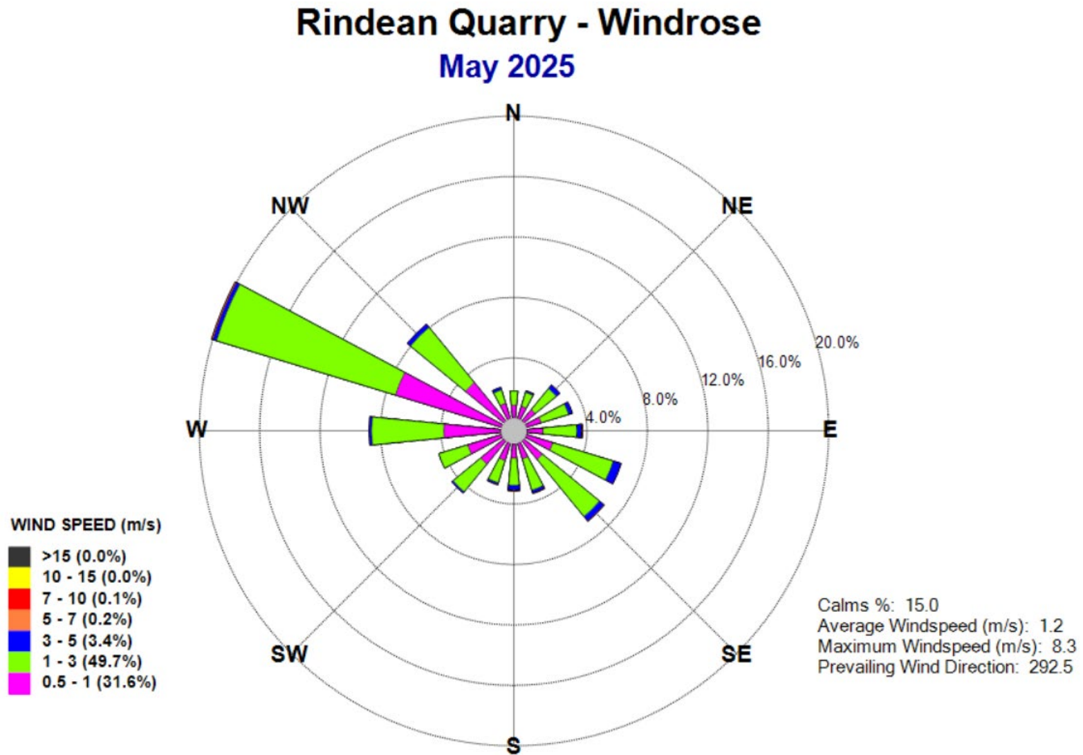
Figure 2: Windrose – May 2025
