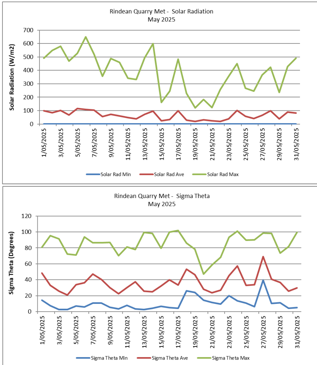
Figure 9-10: Daily (minimum, average, maximum) Solar Radiation and Sigma Theta
