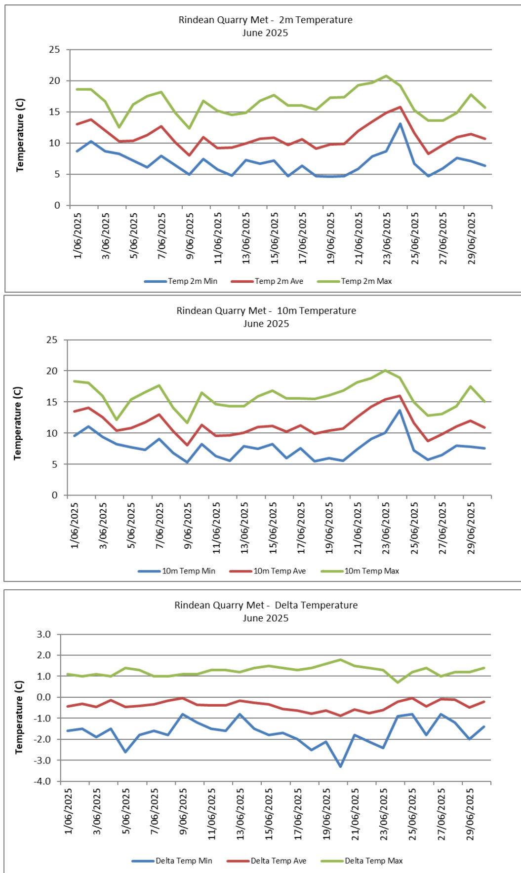
Figure 3-5: Daily (minimum, average, maximum) 2m & 10m Temperature and Delta Temperature
