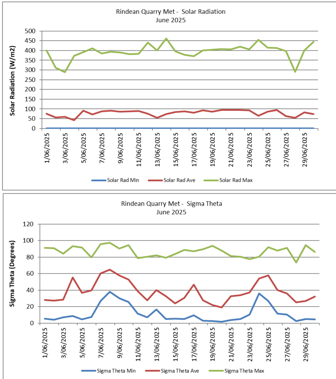
Figure 9-10: Daily (minimum, average, maximum) Solar Radiation and Sigma Theta
