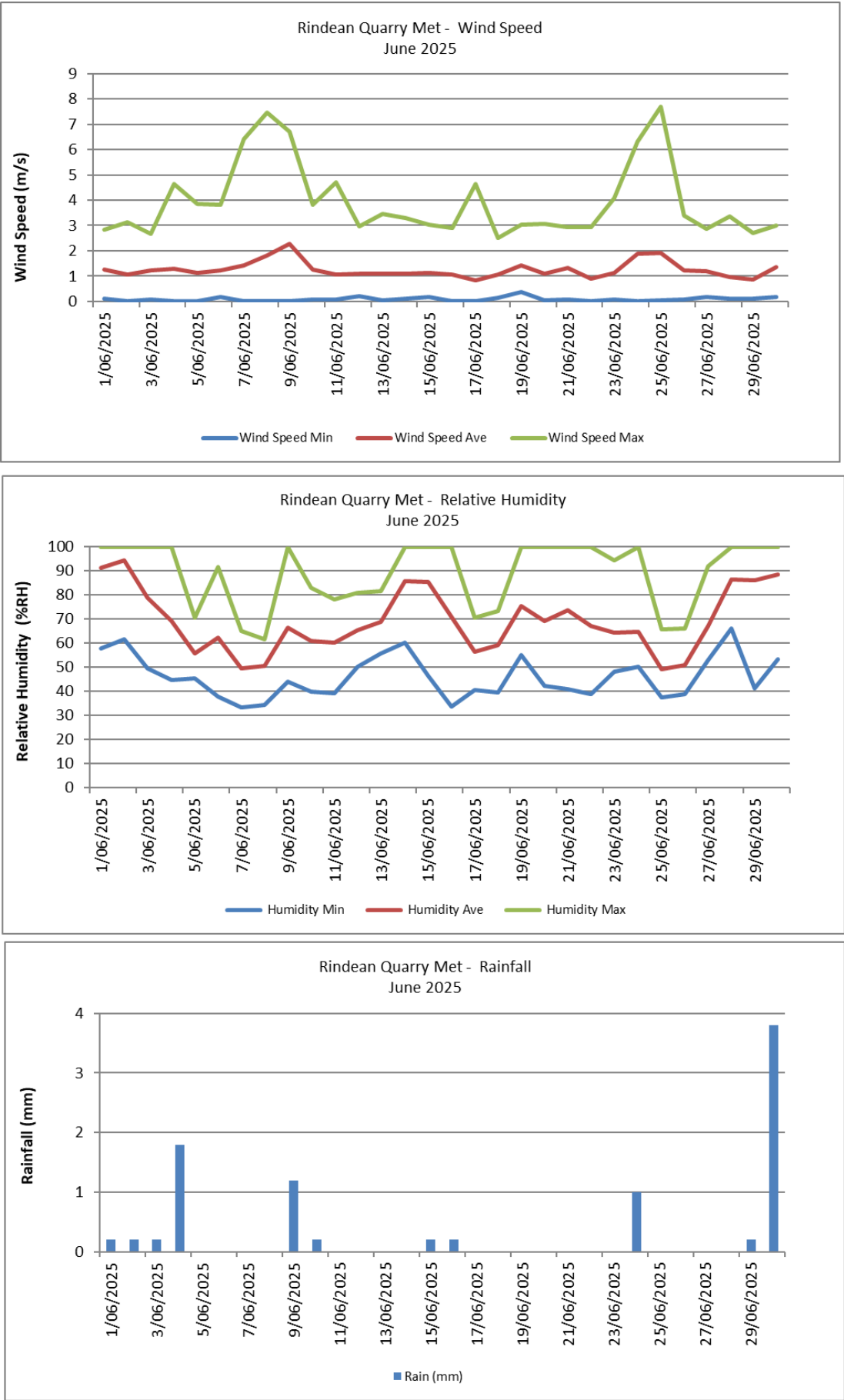
Figure 6-8: Daily (minimum, average, maximum) Wind Speed & Humidity and Rainfall
