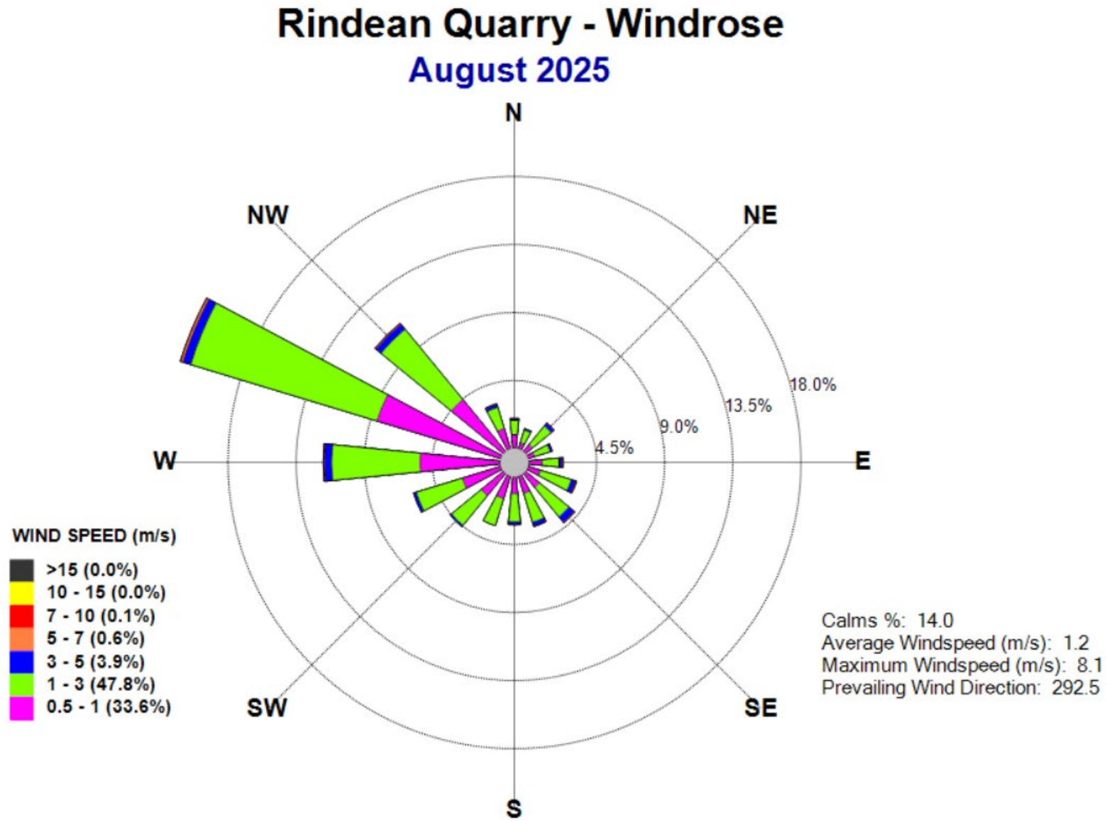
Figure 2: Windrose – August 2025
