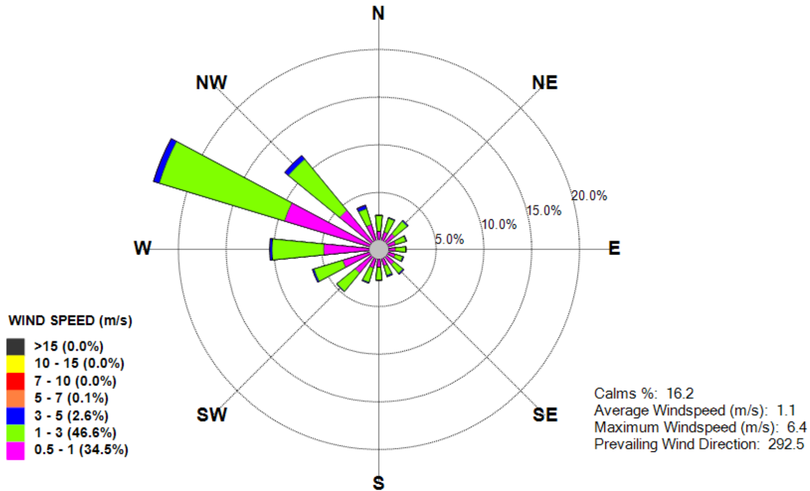
Figure 2: Windrose – July 2026
